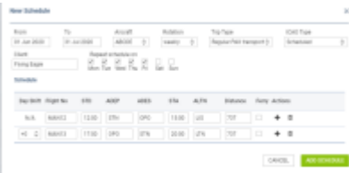
Creating a new schedule in SCHED panel
